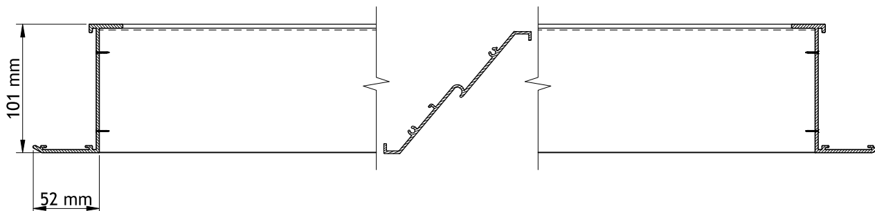
FLANGED FRAME - HORIZONTAL SECTION
