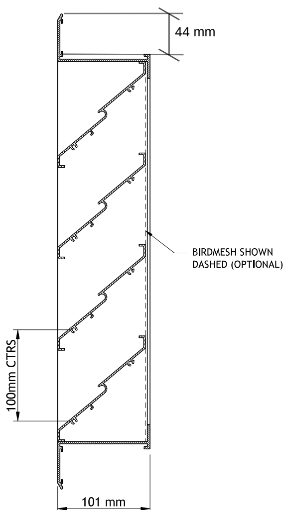
FLANGED FRAME - HORIZONTAL SECTION
